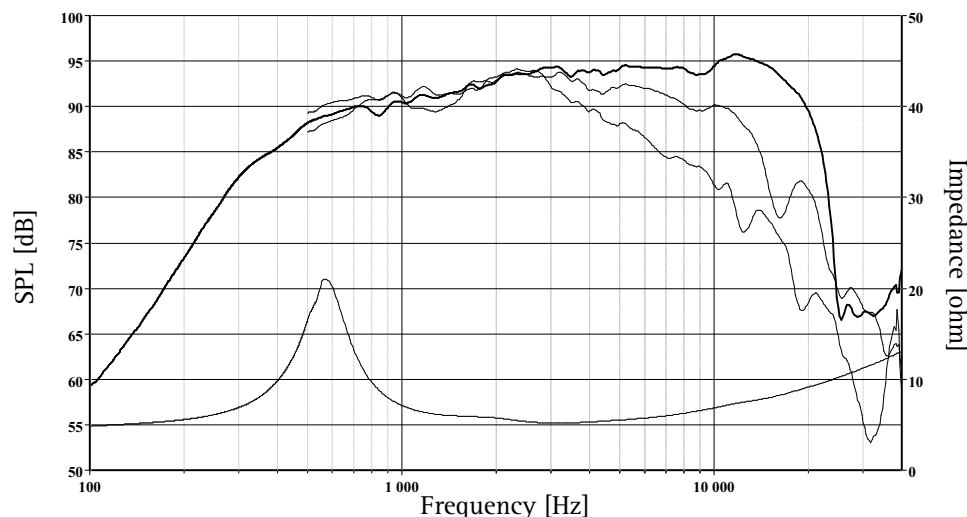
The frequency responses above show measured free field sound pressure in 0, 30, and 60 degrees, mounted in a 0.6m by 0.8m baffle. Input 2.83 Vrms, microphone distance 0.5m, normalized to SPL 1m. The impedance is measured without baffle using a 2V sine signal.
