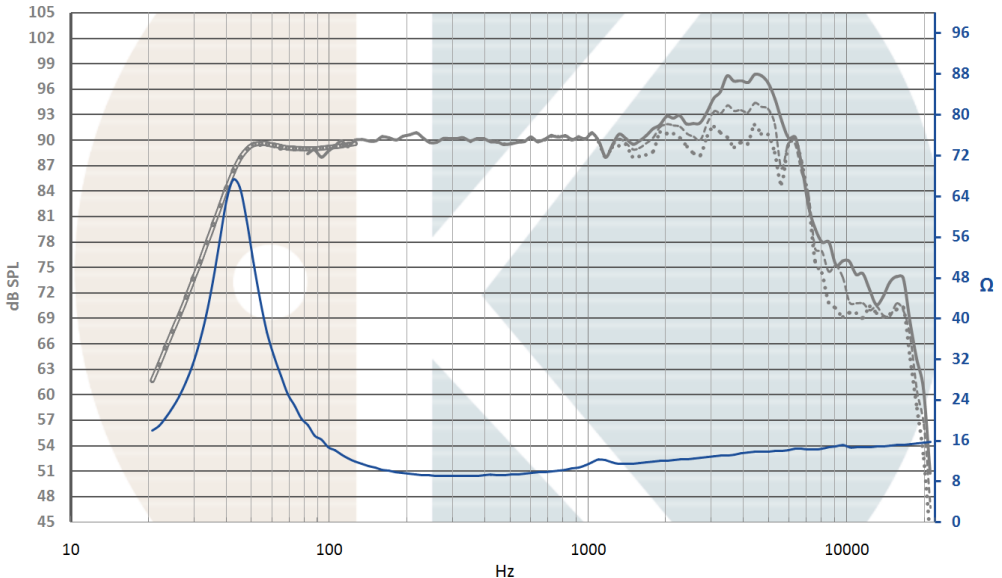
On IEC baffle / Distance: 1m / Signal input: 2,83V / Dash curves: 30° & 60° Impedance measured in free air / Smoothing: 1/12 Octave Curve below 130Hz is simulated in 17L vented enclosure, Fc = 45Hz
