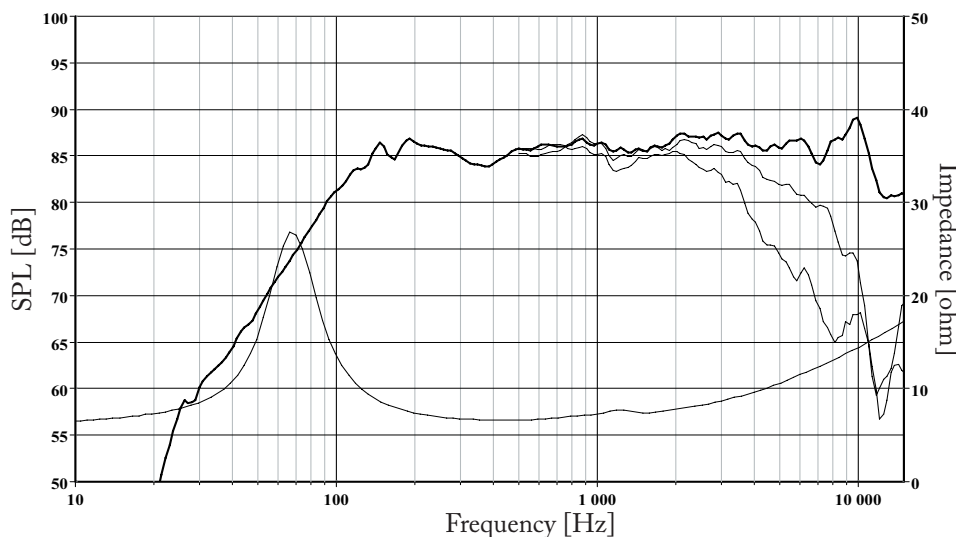
The frequency responses above show measured free field sound pressure in 0, 30, and 60 degrees angle using a 0.8L rear chamber mounted in a standard IEC baffle. Input 2.83 VRMS, microphone distance 0.5m, normalized to SPL 1m. The impedance is measured in free air without baffle using a 2V sine signal.
