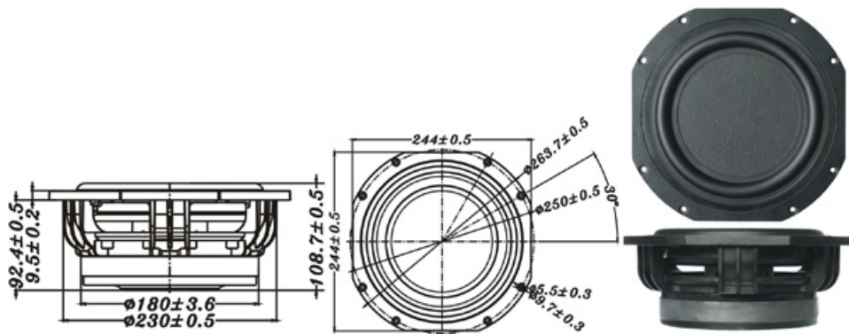
8" PP SANDWICH FOAM WOOFER
