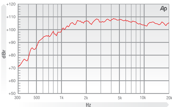
Frequency response measurement taken on axis with 1w signal at distance of 1M using custom horn with 90° x 40° coverage
